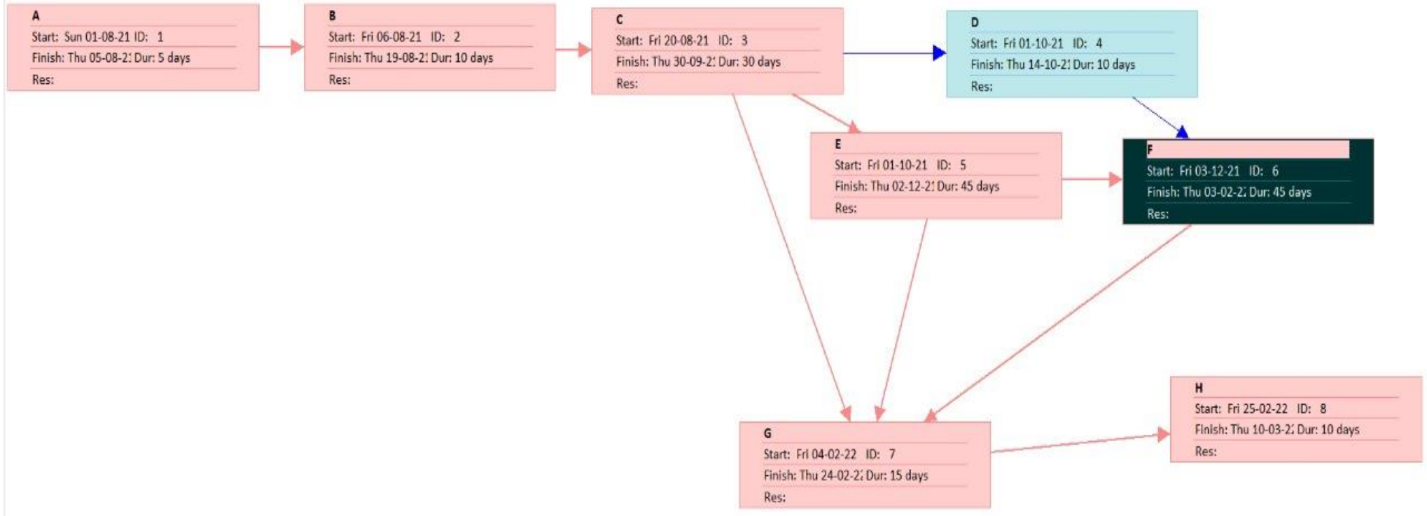
PERT Diagram
